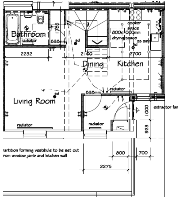
GROUND FLOOR PLAN FLOOR PLANS 1:50
