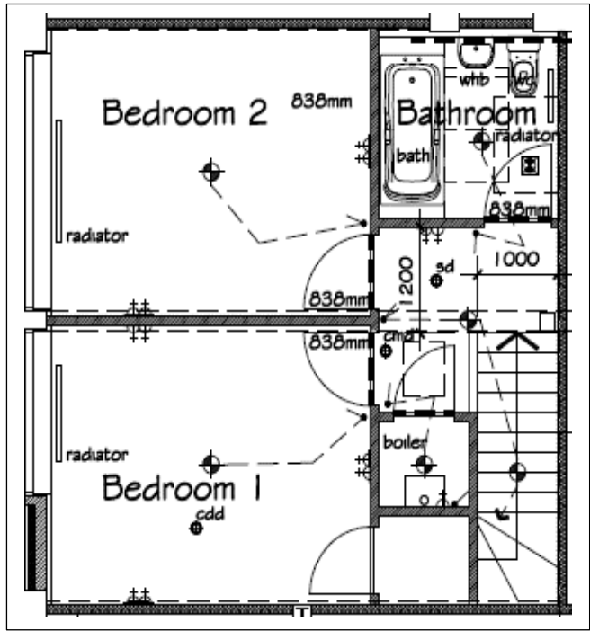
Upper Floor
